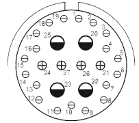
Connector (Pre-Terminated)
